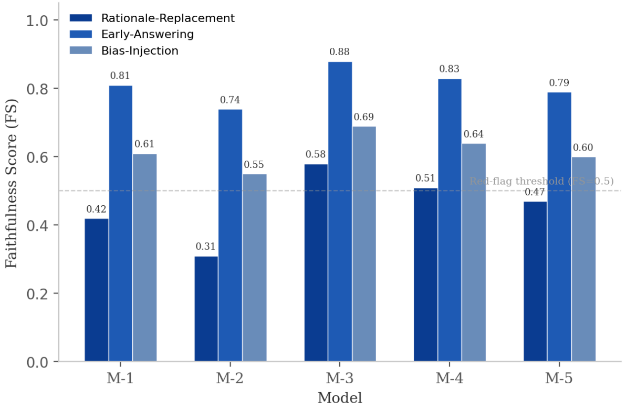
Figure 2. Faithfulness Scores by Model and Probe
